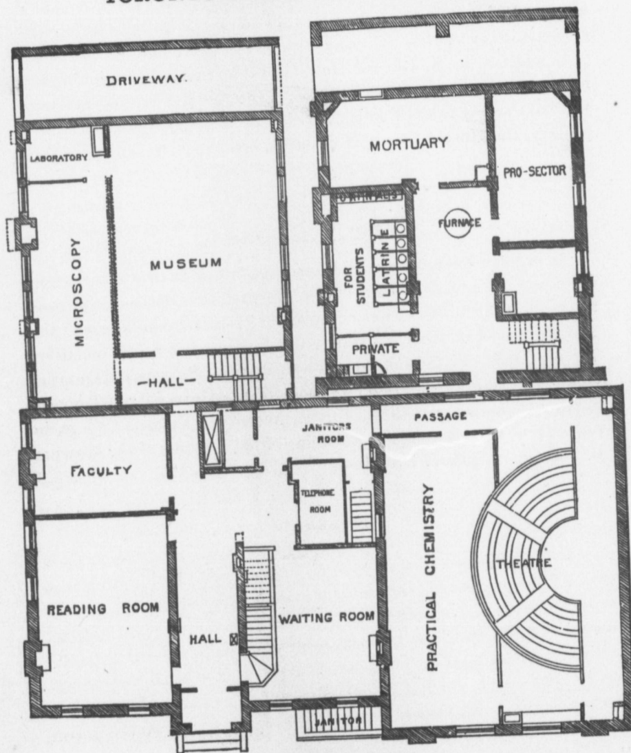
Plan-GROUND FLOOR.
