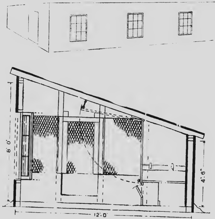
CROSS SECTION.
