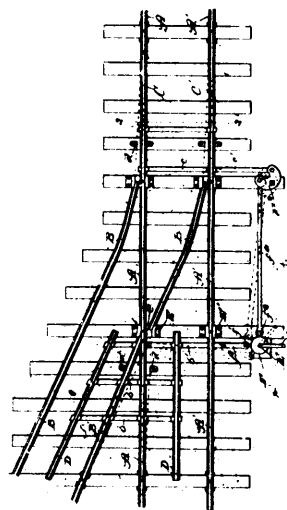
36157 Ackery's Railway Switch.
