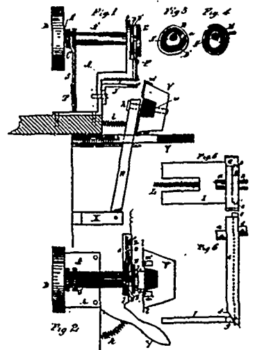
23061 Haines & Wanzler's Machine for Stitching Baskets with Wire.
