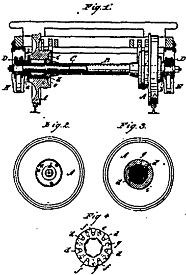
23056 Candee's Running Gear for Railway Cars.
