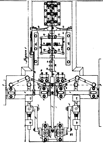
16085 Werts' Improvements in Horse Shoe Nail Machines.
