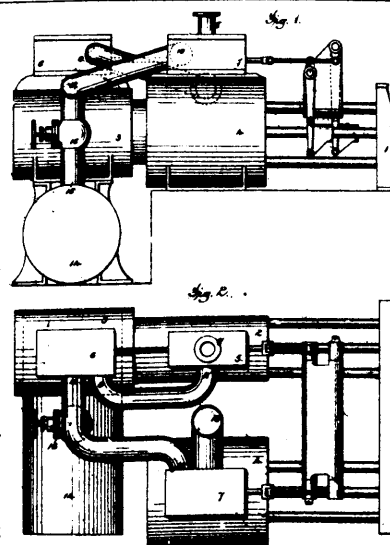
16090 Perry's Improvements on Pumping Engines.
