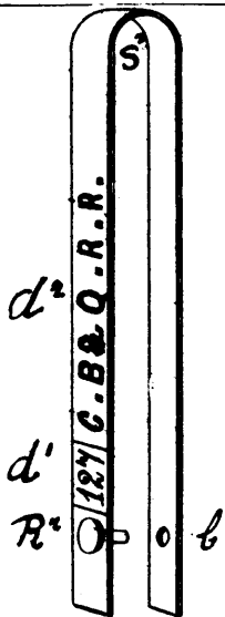
16086 Brooks' Improvements on Seals for Securing Car Doors and other Purposes.
