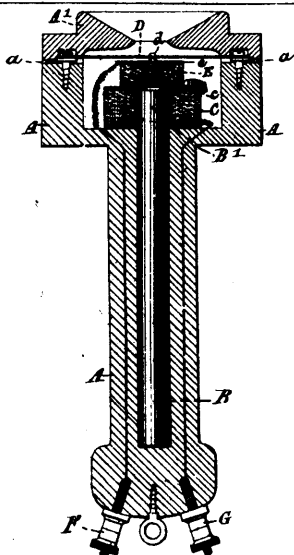
16089 Strangways' Improvements in Telephones.
