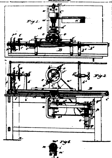
16088 Anderson's Improvements on Moulding Machines.
