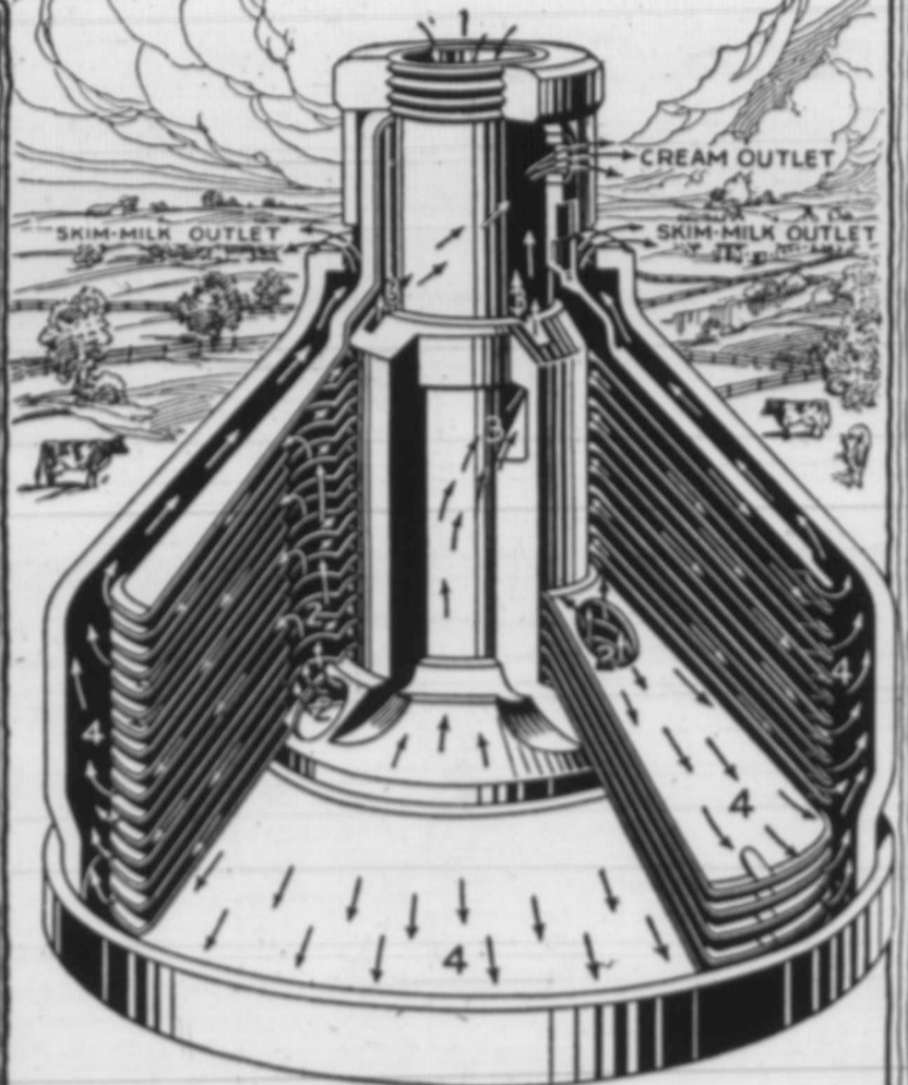
THE NEW SELF-CENTERING, DE LAVAL BOWL
