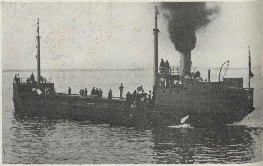
One of three steel steam lighters recently completed at the Polson Shipyard for the Department of Railways and Canals, and for use at Port Nelson Terminals in the Hudson Bay. One illustration shows the lighter being launched, the other shows her ready for use.
