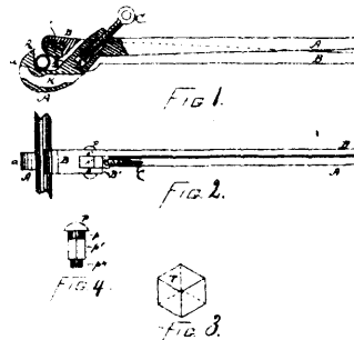
11709 Lovrien's Improvements on Pipe Tong.
