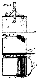
11710 Burtis's Improvements in Mop Wringers.
