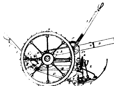
11706 Sweet &amp; Watson's Improvements on Mowing Machines.
