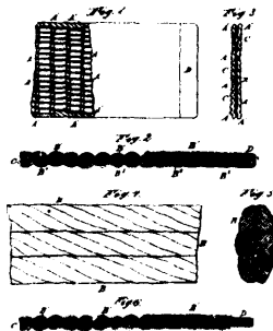
11703 Long's Improvements on Machine Belting.
