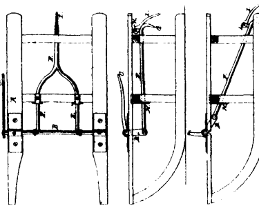
3165 Bromley's Improvements on Sled Brakes.
