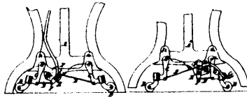
3165 Bromley's Improvements on Sled Brakes.
