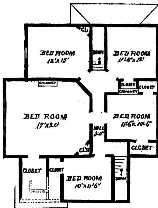
SECOND STORY.
