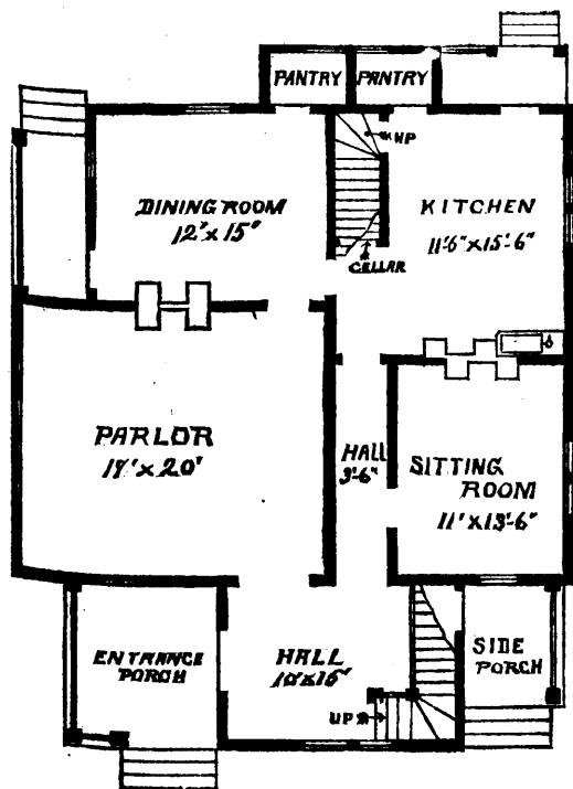
FIRST STORY.
