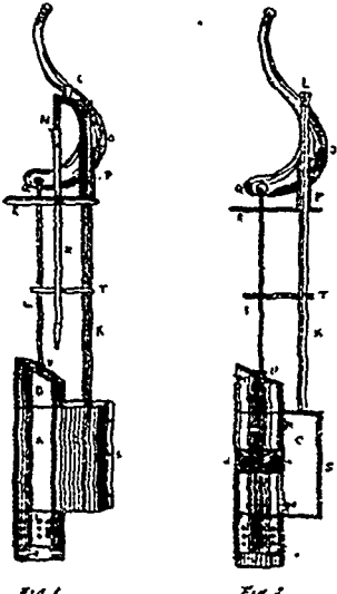
24387 Parker's Force Pump.
