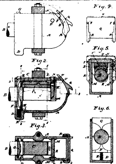
19223 Timm's Car Axle Box.
