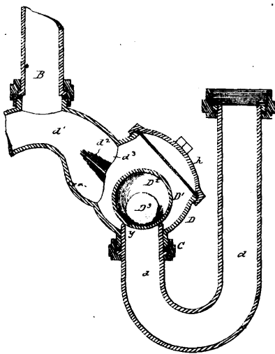
19218 Bennor's Trap for Water Closets, Lavatories, &amp;c.
