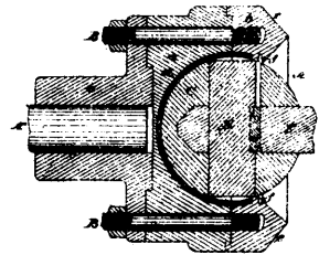
15666 Johnston's Improvements on Coupling Joint for Shafting.
