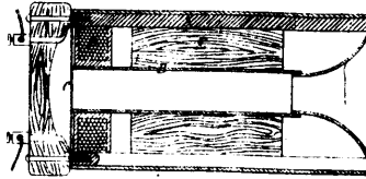
9055 Pole's Improvements in Telephones.
