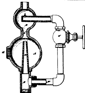
9061 Doty's Steam Water Elevator.
