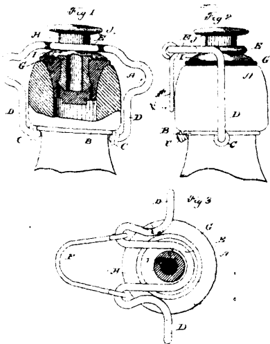
20941 Walter's Bottle Stopper.
