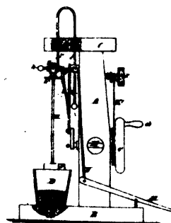
No. 1752. Worthley's Mechanical Motor.
