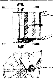
No. 1747. Chamberlain's Manure Cart.
