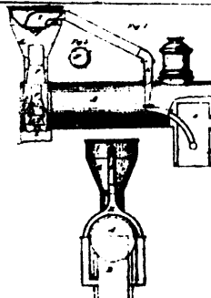
No. 1750. Griggs' Spark Arrestor and Consumer.
