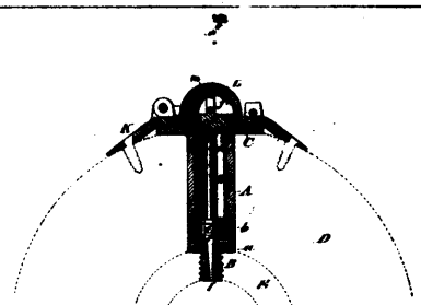
7082 Hertlhey & Dennis' Improvement on Axle Trees.
