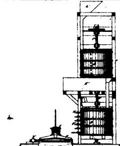
7078 Crosby, Amory, Hannon, Wetherbee, Mitchell & Beate's Process and Apparatus for Treating the Ores of Gold and Silver.
