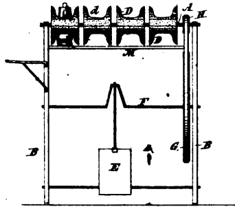
7072 Laurie's Apparatus for Cleaning and Polishing Boots and Shoes.
