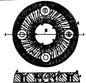
5386 Howland's Metallic Grinding Ring Dress.
