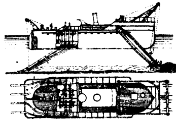
5375 Bazin's Improvements on Dredging Boats.
