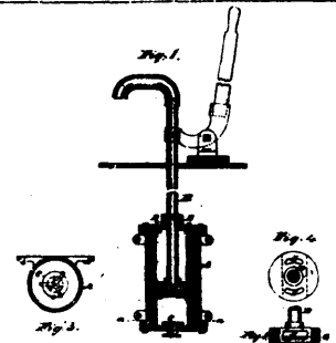
5376 Riddell's Improvements on Suction and Force-pumps.
