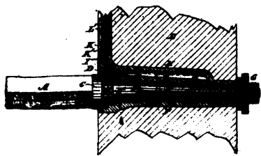
5384 Payette's Improvements on Axles and Axle-boxes.
