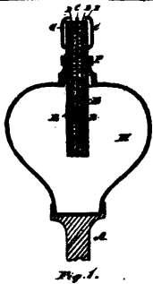
5377 Benson's Improvements in Lamp Burners.
