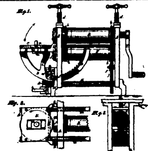
5383 Nugent & McGregor's Machine for Turning Flanges on Boiler Heads.
