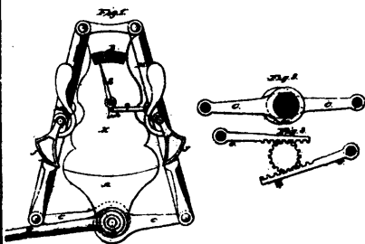
5380 Hobbs' Tire-shrinking Machine.
