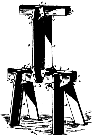
22631 Zeigler's Socket Clamp for Trestring and Scaffolding.
