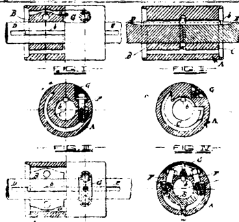
11916 Walker's Improvements on Shaft Couplings.
