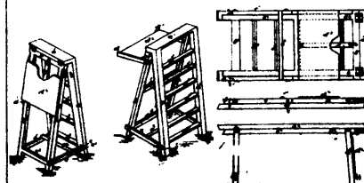
5162 Hood's Combined Ladder and Wash Bench.
