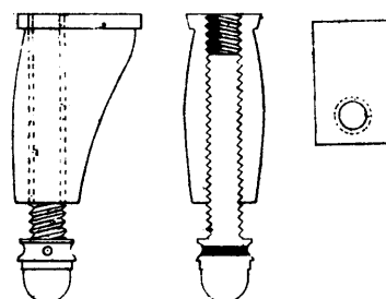
5149 Wheeler's Improvements on Stove Legs.
