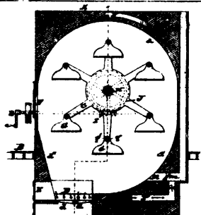
5147 Hall's Improvements in Revolving Reel Baking Ovens.
