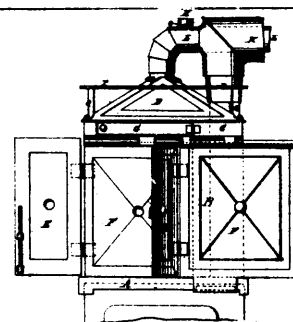
5146 Smedley's Improvements on Cooking Stoves.
