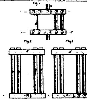
4298 Hutchinsen's Heating Drum.
