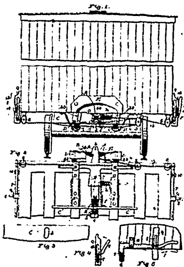
29679 Barry's Car Coupling.
