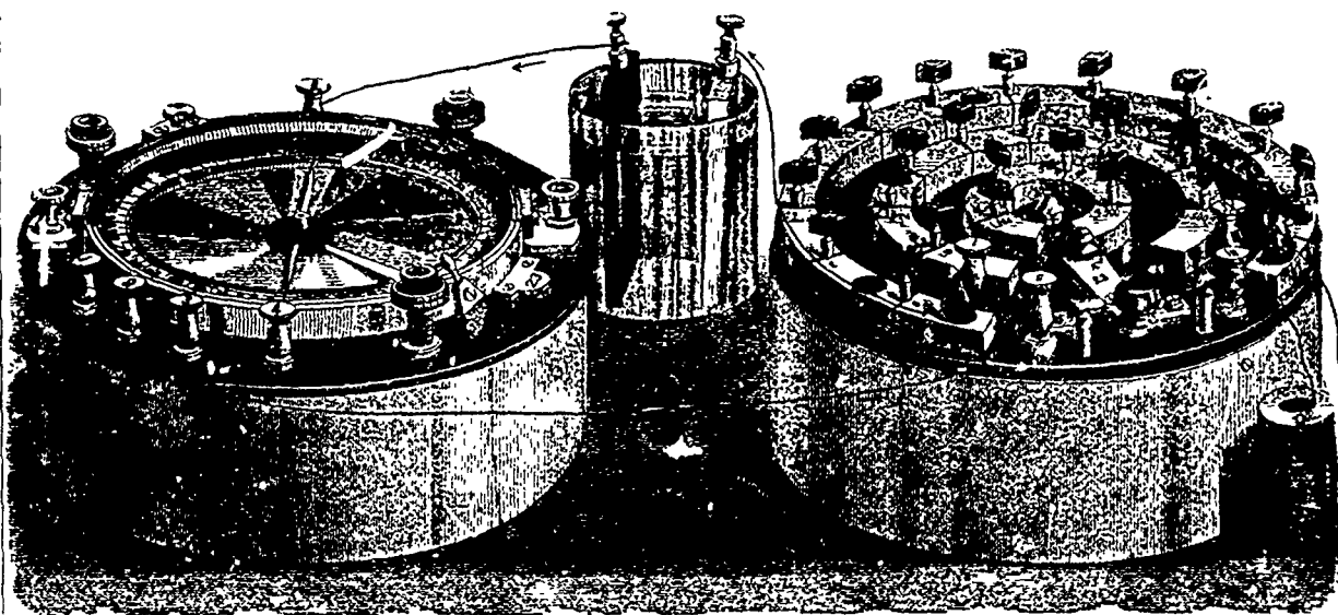
BRADLEY'S APPARATUS FOR ELECTRICAL MEASUREMENT (See page 102.)
