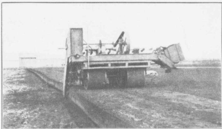
Dobson's peat excavator; front view.
