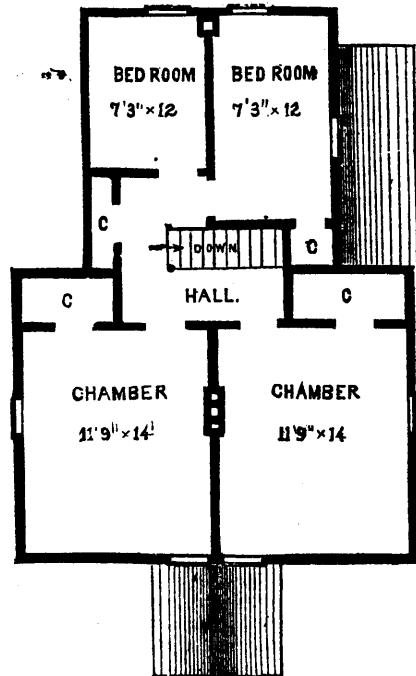
Fig. 3.—PLAN OF SECOND STORY.
