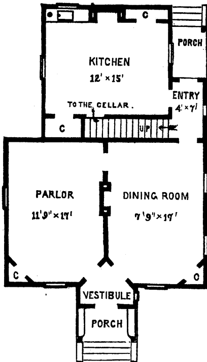
Fig. 2.—PLAN OF FIRST STORY.
