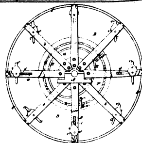
5484 Forward's Improvements in Paddle Wheels.
