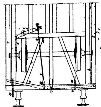
35069 Panter, Taite and Carlton's Vehicle Brake.
