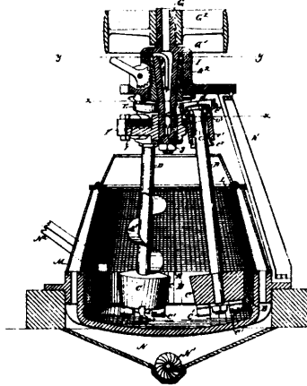
35062 Rice's Pulverizing Mill.
