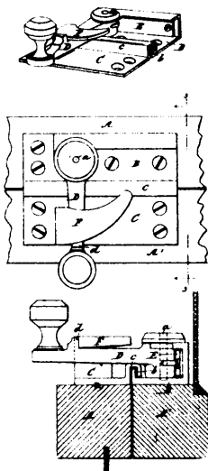
Pardoe's Sash Fastener.
