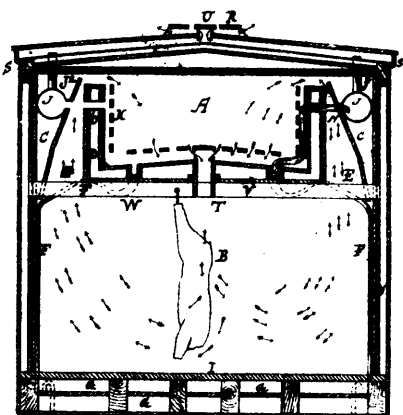
Cook's Refrigerator Car.
