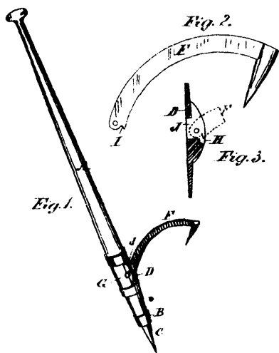
McLean's Cant Hook.
