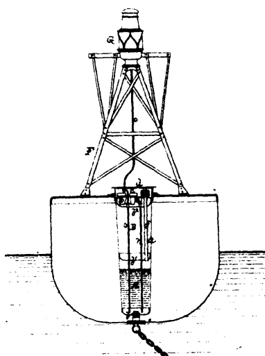
Pinch's Illuminating Apparatus.
