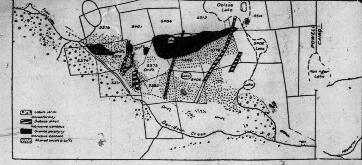
Sketch of the "Boat Structure" as developed in the Quartz Porphyries and Diabases of Northern Ontario.
