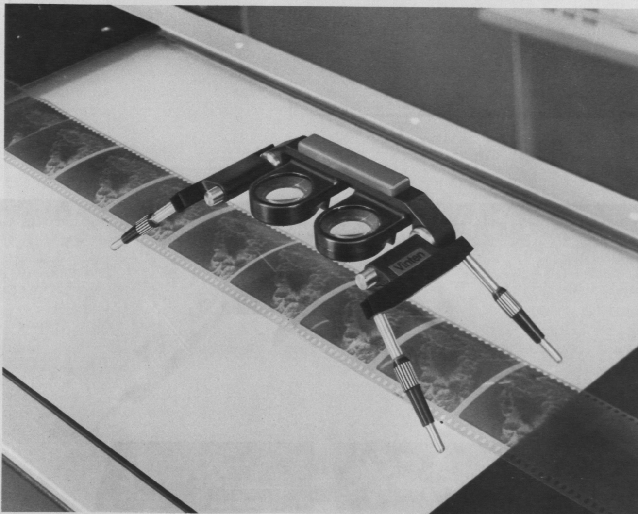
Figure 13. Lens stereoscope with 2x and 4x magnification lenses. (Courtesy of Vinten Military Systems Ltd.)
