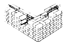
Corrugated Ties for Hollow Wall Construction
