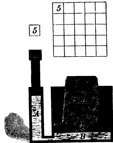
FIG. 6.—PRINCIPLE OF HYDRAULIC PRESS.
