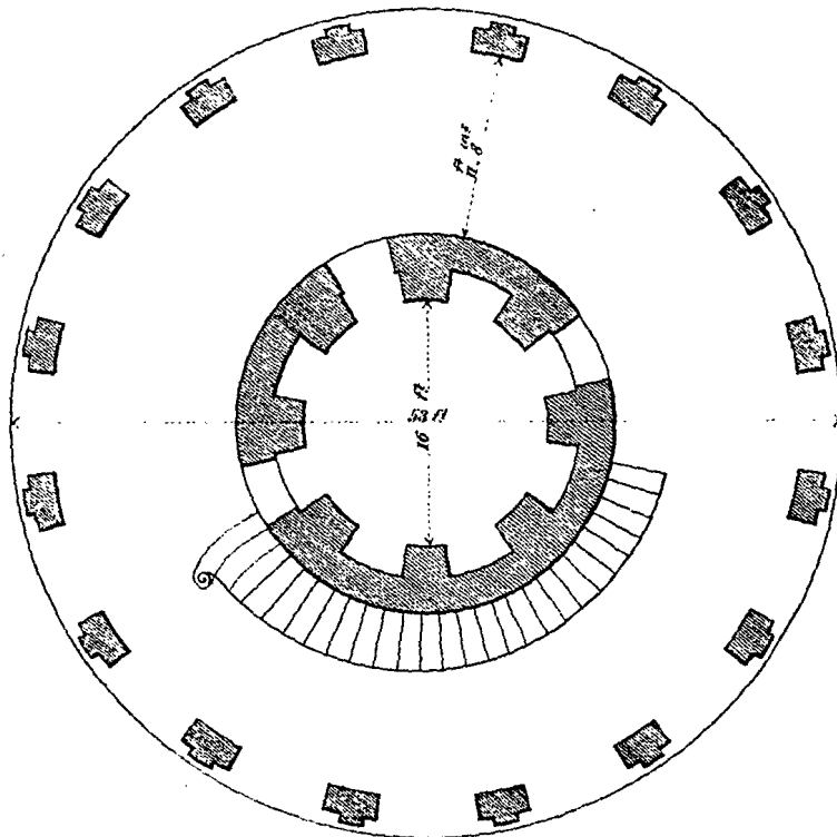
GROUND PLAN.
