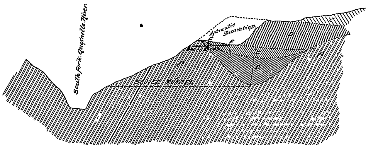
Sketch Showing Geological Section on Line Across Workings in the China Pit, Cariboo Hydraulic Mine, B.C.
