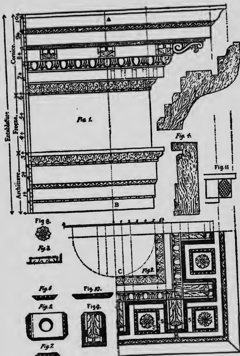
ELEVATION OF CORINTHIAN ENTABLATURE AND PLAN OF CORNICE AT EXTERNAL ANGLE. PLATE I
