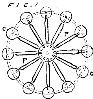
BARNEY'S IMPROVEMENTS IN TELEPHONES.
