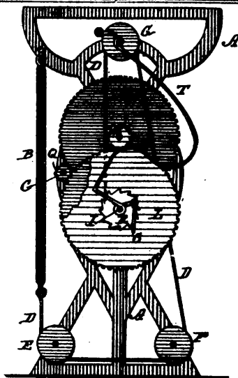
Wright's Spring Motor.
