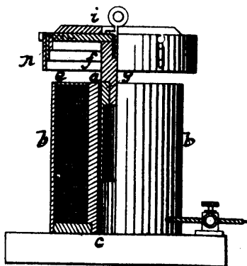
Timmis & Currie's Electro-Magnet and Armature.
