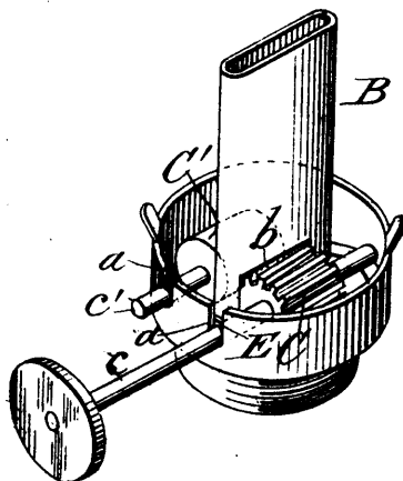
Ream's Lamp Burner.
