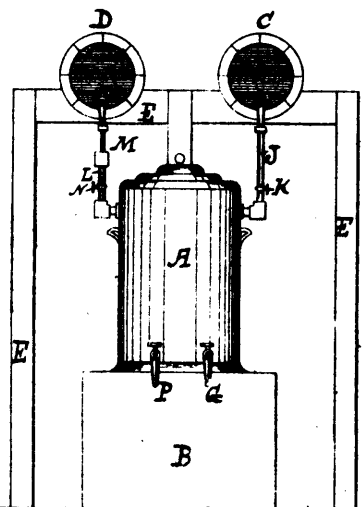
Bartliff's Beer Cooler.
