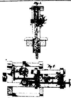
11811 Cilley's Improvements on Saw-mills.
