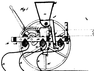
11804 Springer's Improvements in Cultivators and Seeders.
