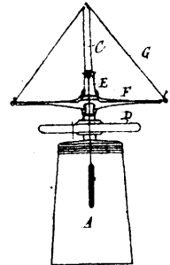
11806 Ryckman's Improvements in Rotary Churns.
