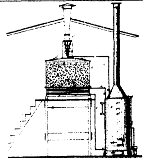
11809 Scholheid's Apparatus for Drying Coffee, Fruit and other Materials.
