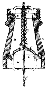
11808 Woodruff's Improvements on Gas Regulators.
