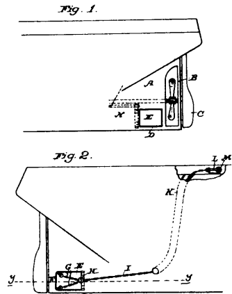
42003 Weitzel's Auxiliary Steering Gear.
