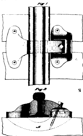
36228 Sintzenich's Railway Rail Chair.
