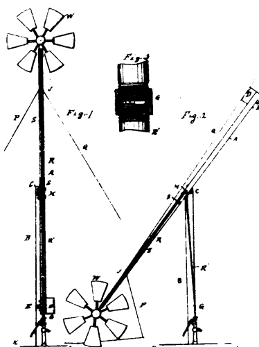
30788 Perry's Wind Mill Derrick.
