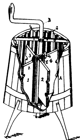
30795 Jones' Washing Machine.
