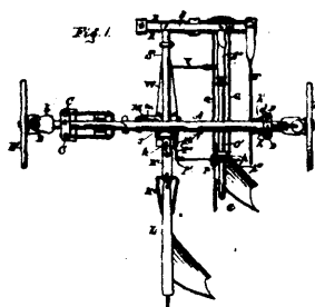
13190 Holgate's Improvements on Gang Ploughs.
