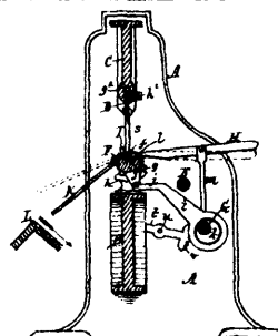
13188 Greenwood's Improvements on Hoop Cutting Machines.
