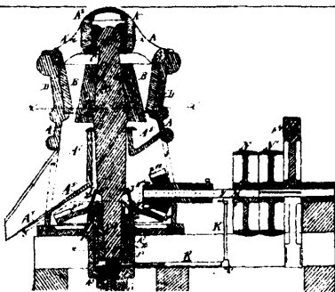
13178 Gates's Improvements on Machines for Breaking and Crushing Stones.
