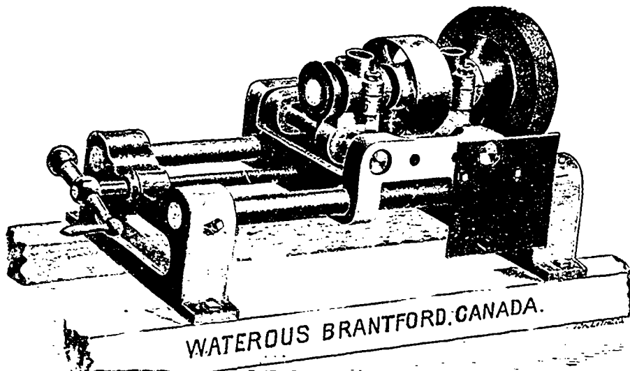
Band Wheel Grinding Machine For Grinding and Truing Up Face of BAND MILL WHEELS in Mill.
