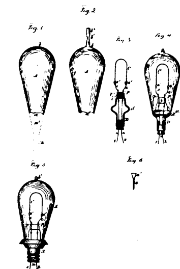
15844 Edison's Improvements on Electric Lamps.
