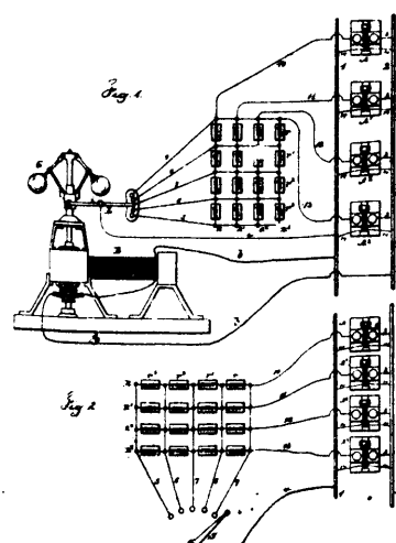
15848 Edison's Improvements on Regulators for Magneto or Dynamo-Electric Machines.
