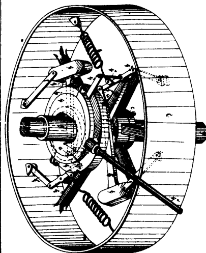
15842 Ball's Improvements in Steam Engine Governors.
