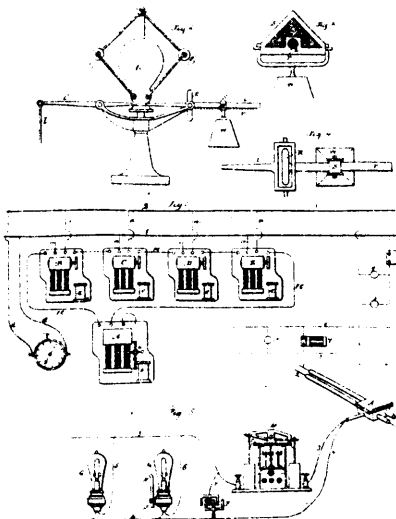
15846 Edison's Improvements on Regulators for Magneto or Dynamo-Electric Machines.
