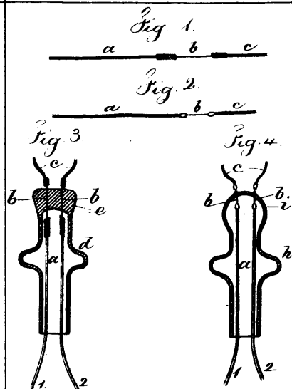
15845 Edison's Improvements on Electric Lamps.
