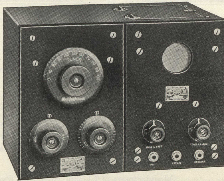
Westinghouse Type R. C. Receiving Set
