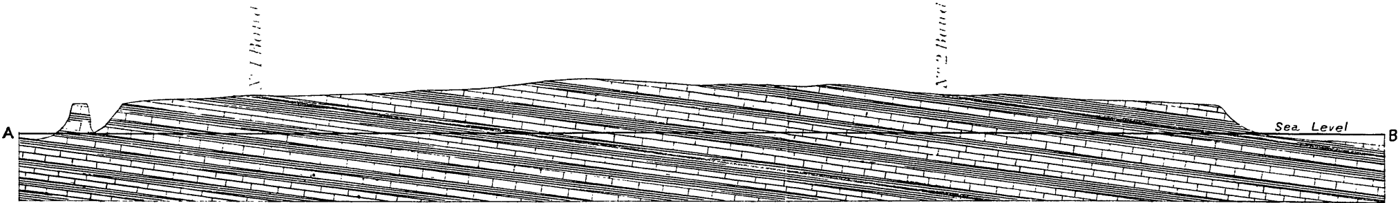
SECTION A.B. SHOWING POSITION OF ORE BANDS Nos 1 & 2
