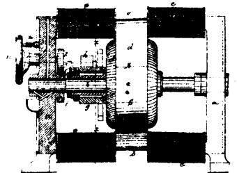
15539 Wood's Improvements on Electric Generators.
