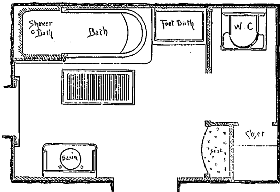
Plan
